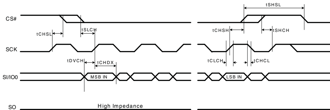
Figure 9.4 Input Timing
